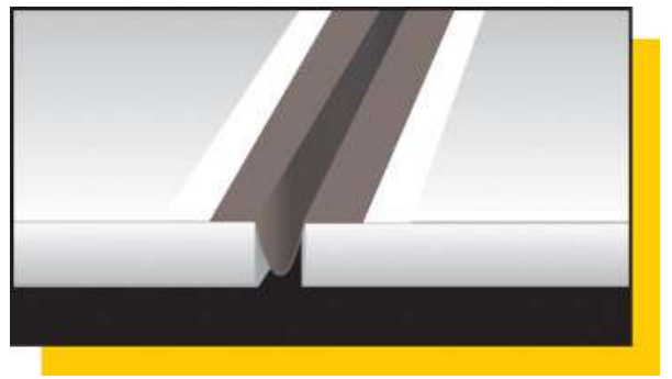
Positioning Mapeband PE 120 in an omega pattern in an expansion joint
