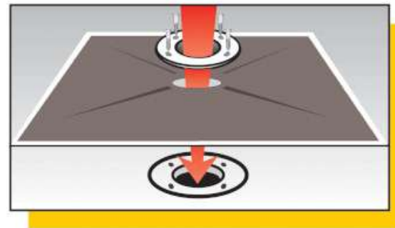
Square PVC element for flexible waterproofing and sealing of a 425 mm x 425 mm drain
